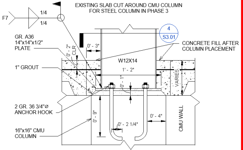
7 COLUMN CONNECTION FROM SIDE 1 1/2" = 1'-0"
