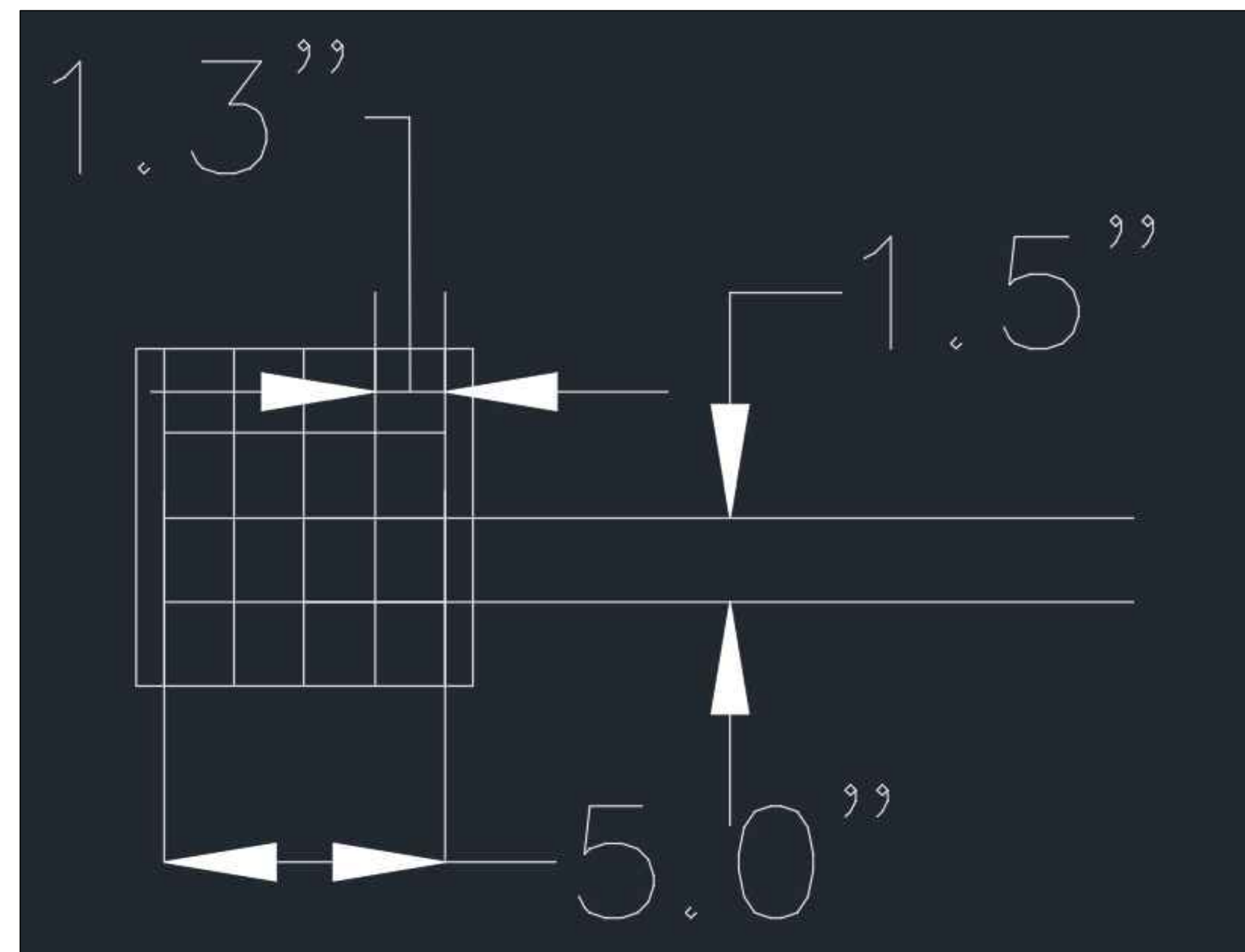
5' Rebar Cross Section
