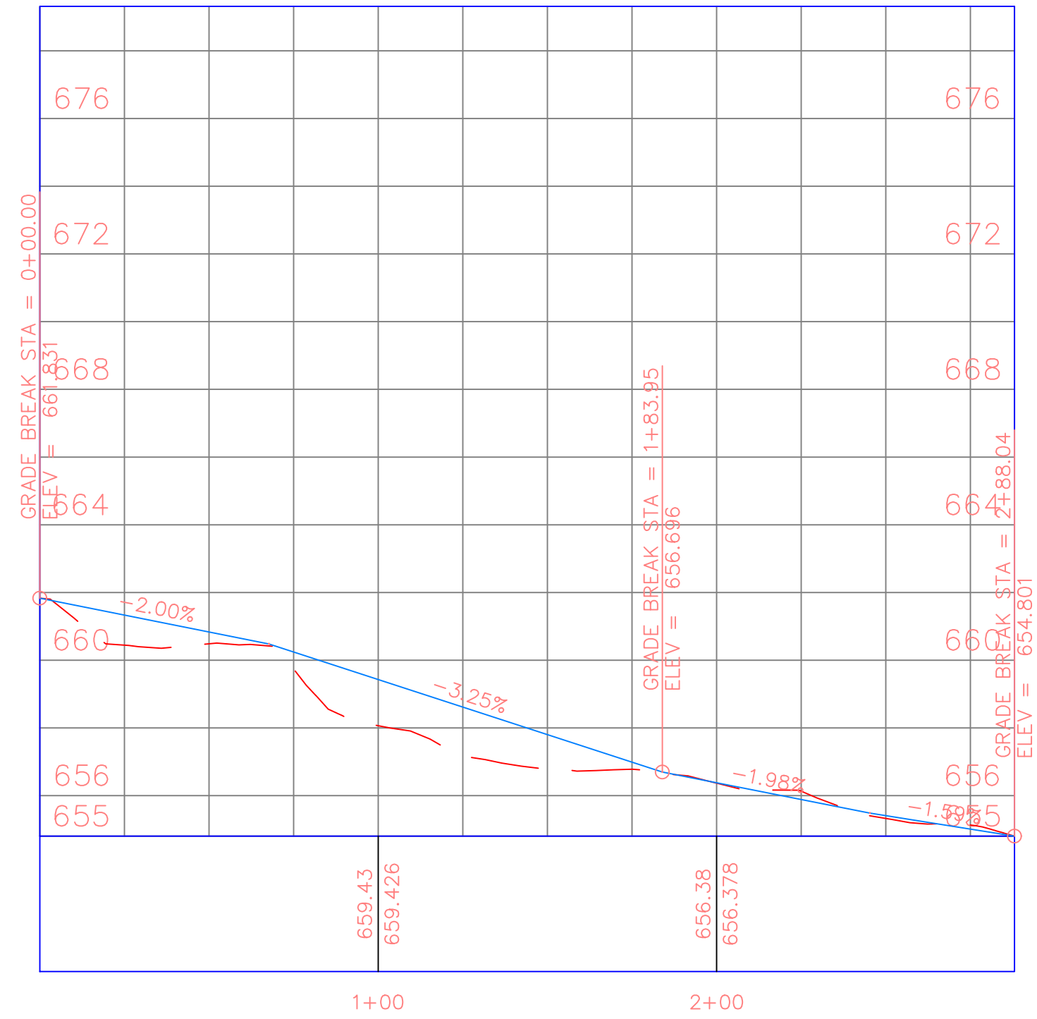
CC Horz Alt 4 PROFILE
